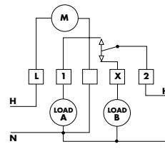
W120 (SPDT)
