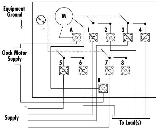
W400A (4PST)
