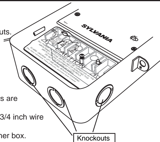
Outdoor timer case
