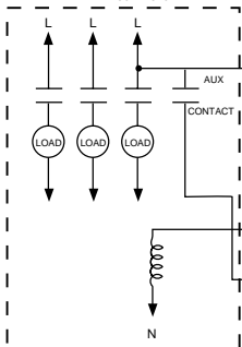
ELECTRICALLY HELD CONTACTOR MOTOR STARTER
