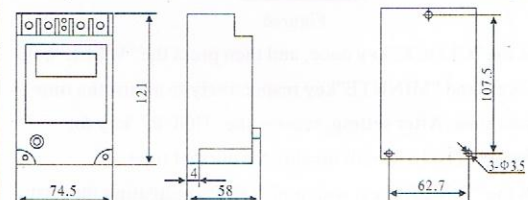
a) Physical dimension of KG316T b) Opening size of KG316T
