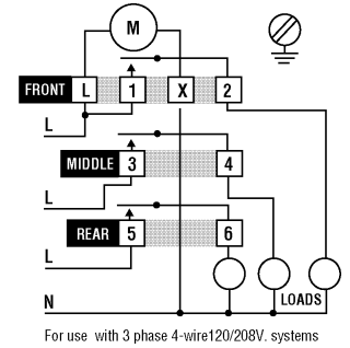
For use with 3 phase 4-wire 120/208V. systems
