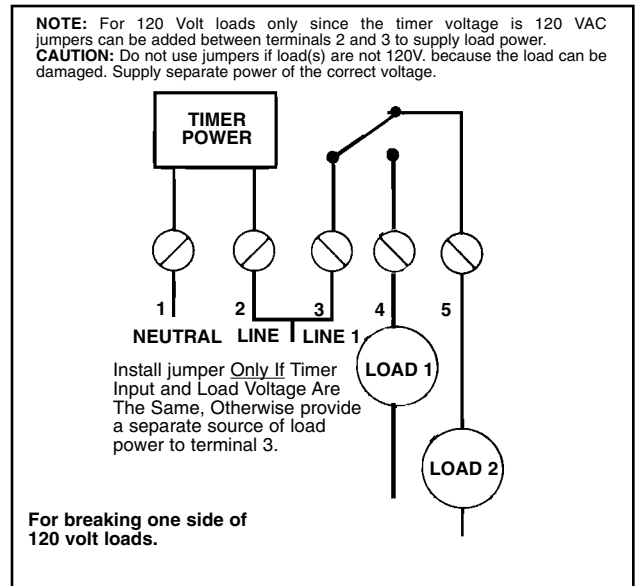
FIG. #5 ET105C SPDT
