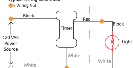
Typical Wiring Schematic
