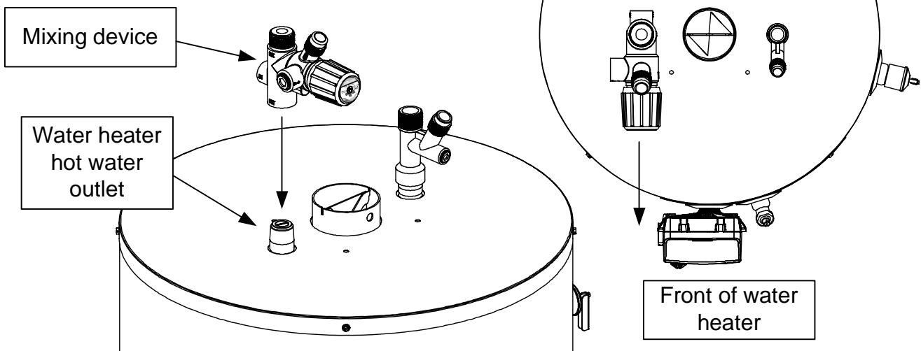
Figure 6 Installing Mixing Device
