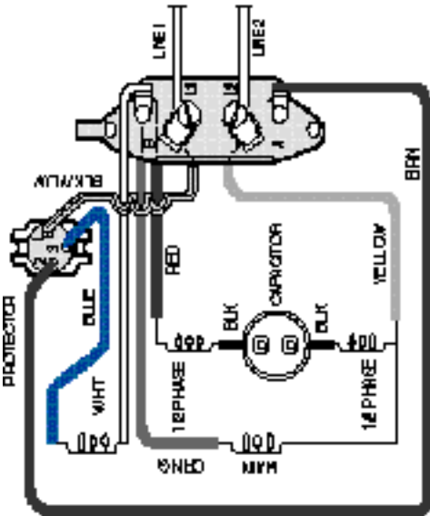
Wiring Diagram #16635902. Connection Label #17536715.
