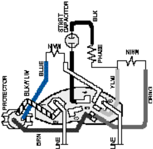
Wiring Diagram #157682. Connection Label #161035.
