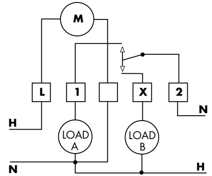
7120Z (SPDT)
