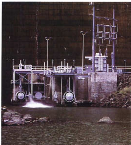
A small hydroelectric installation at the base of the Monticello Dam west of Sacramento, California, exploits a high head (about 400 feet) to extract about 11 megawatts of energy from a modest flow of water. The turbine is a Francis wheel, a hybrid type that draws on both the impulse and the reaction principles. The discharge is above the level of water in the tailrace.
