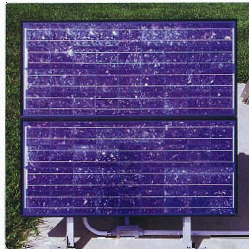
Photovoltaic cells, which generate electricity directly from sunlight, are made of polycrystalline silicon. The array of cells above is installed at Montgomery College in Germantown, Maryland. A detail, below, shows the grain structure of the silicon material and the grid of metallic conductors laid down over it to collect current.
