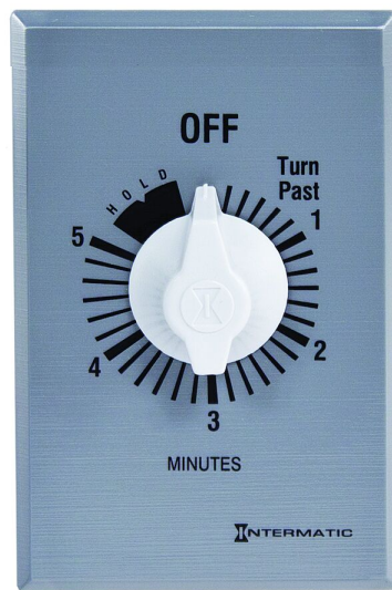
Spring Wound Countdown Timer, Commercial, 125-277 VAC, 50/60 Hz SPST 5 Minute Max, With Hold, Silver
