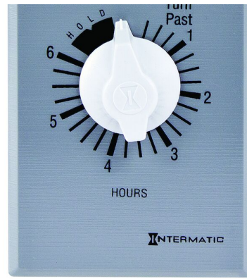
Spring Wound Countdown Timer, Commercial, 125-277 VAC, 50/60 Hz SPST, 6 Hour Max, With Hold, Silver
