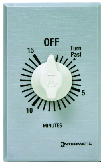
Spring Wound Countdown Timer, Commercial, 125-277 VAC, 50/60 Hz SPDT, 15 Minute Max, Without Hold, Silver
