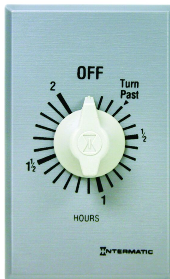
Spring Wound Countdown Timer, Commercial, 125-277 VAC, 50/60 Hz SPDT, 2 Hour Max, Without Hold, Silver
