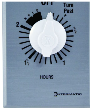
Spring Wound Countdown Timer, Commercial, 125-277 VAC, 50/60 Hz SPDT 2 Hour Max, With Hold, Silver
