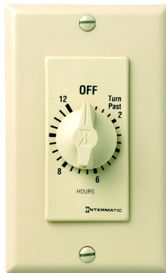
Spring Wound Countdown Timer, Decorator Style, 125-277 VAC, 50/60 H , SPST, 12 Hour Max, Without Hold, Ivory
