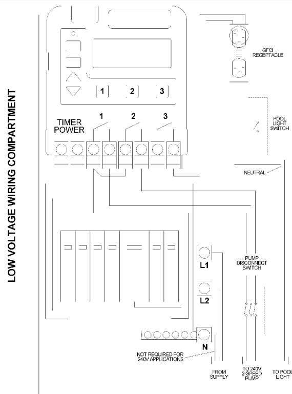
Wiring Guidelines for Modes 2 & 4
