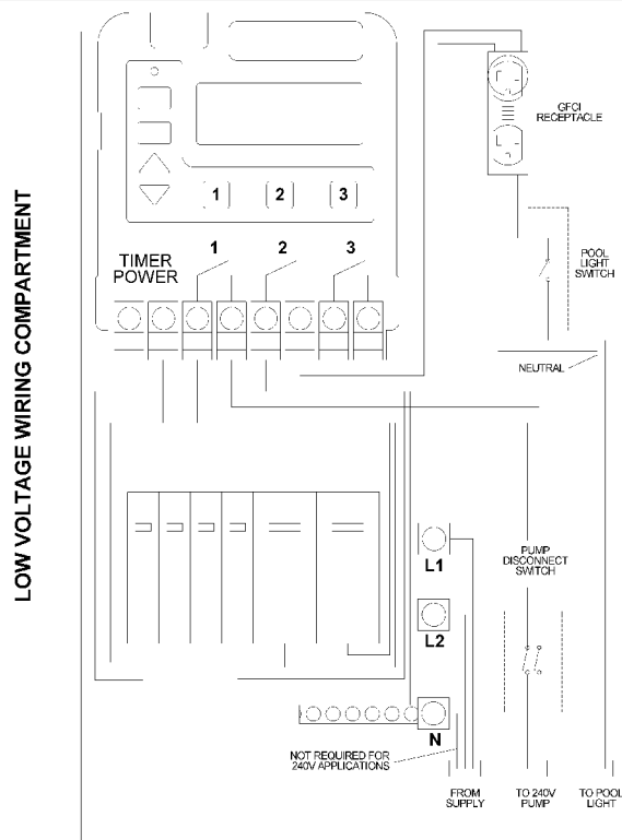
Wiring Guidelines for Modes 1 & 3 (Circuit 3 can be wired similar to Circuit 1)
