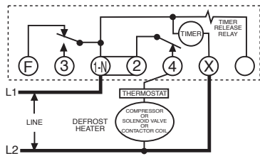
DTMV40 Time/Time–Electric or Air Defrost Wiring Diagram
