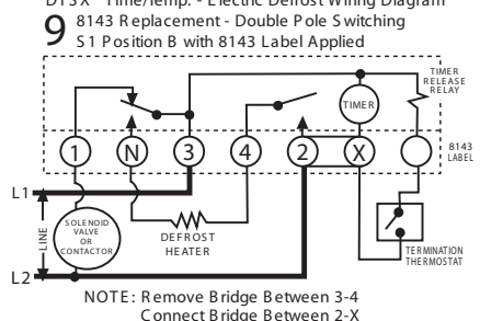
DTSX Time/Temp. - Electric Defrost Wiring Diagram
