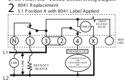
DTSX Time/Time - Electric Defrost Wiring Diagram
