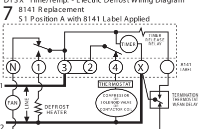
DTSX Time/Temp. - Electric Defrost Wiring Diagram
