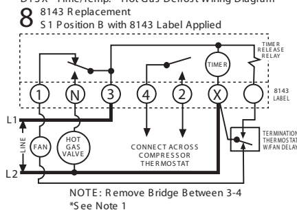
DTSX Time/Temp. - Hot Gas Defrost Wiring Diagram
