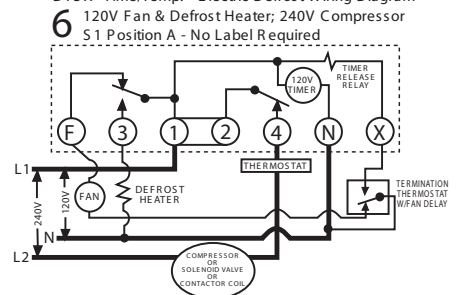
DTSX Time/Temp. - Electric Defrost Wiring Diagram
