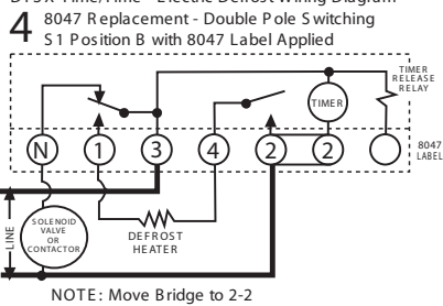
DTSX Time/Time - Electric Defrost Wiring Diagram
