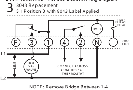
DTSX Time/Time - Hot Gas Defrost Wiring Diagram
