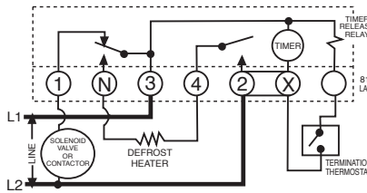
DTMV40 Time/Temperature–Electric Defrost Wiring Diagram
