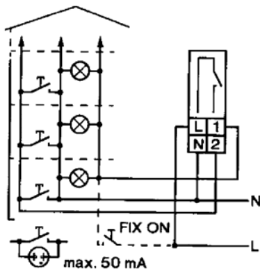
Wiring diagram
