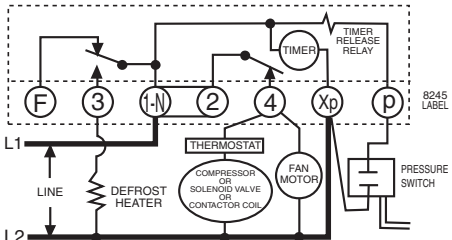
DTMV40 Time/Pressure–Electric Defrost Wiring Diagram 10 8245 Replacement Mode A with 8245 Label Applied
