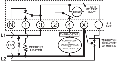
DTMV40 Time/Temp.–Electric Defrost Wiring Diagram 7 8141 Replacement Mode A with 8141 Label Applied
